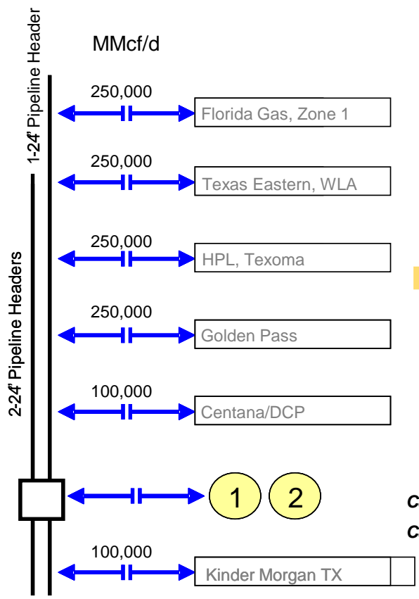
Pipeline Interconnections from West to East
